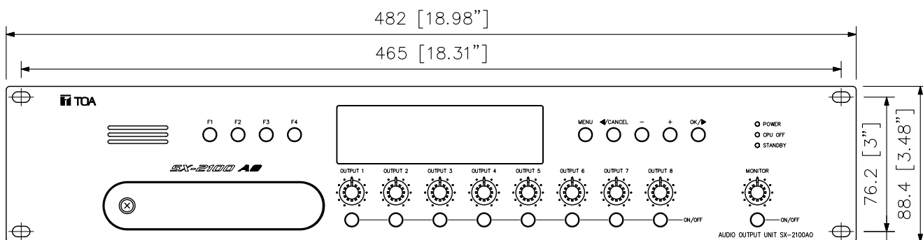
Front View
