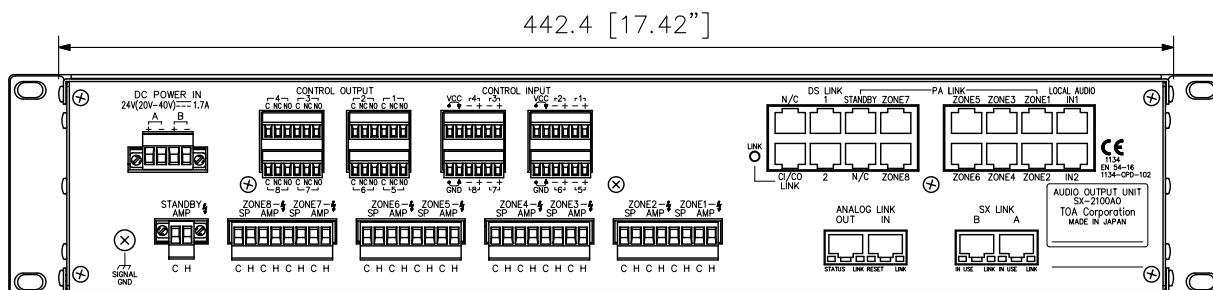
Rear View
